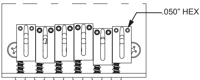
SADDLE HEIGHT SET SCREWS
