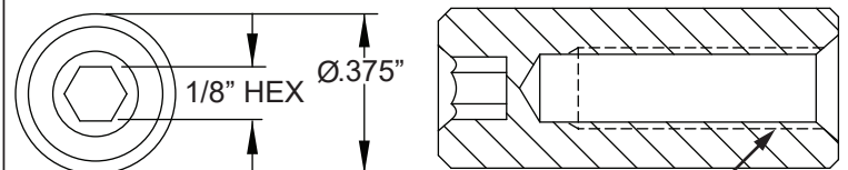
10-32 THREAD
